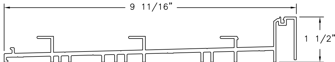
㉖ 3 TRACK HEAD 6063-T6 ALUMINUM 0.115" THICK
