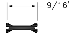
THERMAL I-STRUT NYLON POLYAMIDE 0.070" THICK (66GF25) TENSILE STRENGTH: 10,390 PSI
