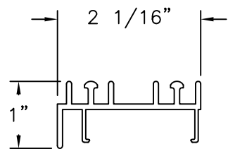
㉚ SILL SCREEN ADAPTER 6063-T6 ALUMINUM 0.080" THICK
