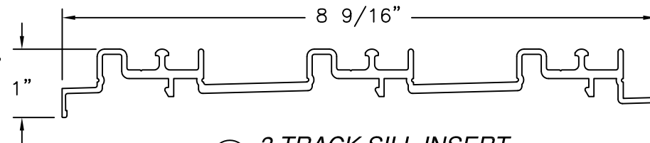
㉙ 3 TRACK SILL INSERT 6063-T6 ALUMINUM 0.125" THICK
