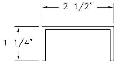
㉓ REINFORCEMENT 6063-T6 ALUMINUM 0.125" THICK
