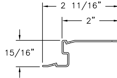
㉔ FIXED PANEL CLIP 6063-T6 ALUMINUM 0.50" THICK
