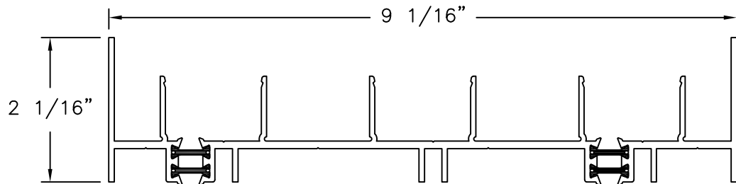
㉖ 3 TRACK HEAD 6063-T6 ALUMINUM 0.115" THICK
