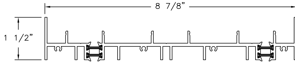
㉗ 3 TRACK JAMB 6063-T6 ALUMINUM 0.115" THICK
