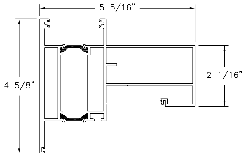
⑭ FEMALE BUTT STILE 6063-T6 ALUMINUM 0.080" THICK
