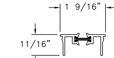
⑤ HEAD INSERT 6063-T6 ALUMINUM 0.050" THICK
