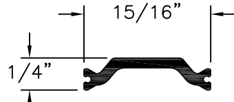
THERMAL I-STRUT NYLON POLYAMIDE 0.070" THICK (66GF25) TENSILE STRENGTH: 10,390 PSI
