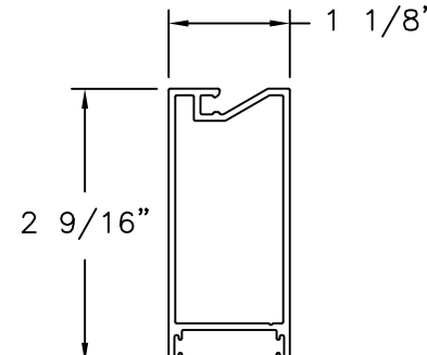
㉞ SCREEN STILE 6063-T6 ALUMINUM 0.062" THICK
