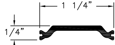
THERMAL I-STRUT NYLON POLYAMIDE 0.070" THICK (66GF25) TENSILE STRENGTH: 10,390 PSI
