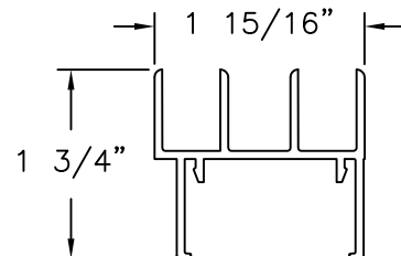
㉛ HEAD SCREEN ADAPTER 6063-T5 ALUMINUM 0.075" THICK
