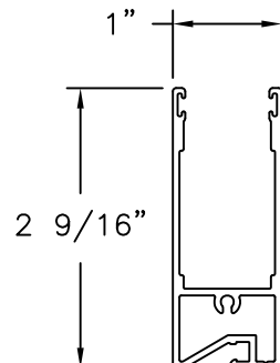
㉝ SCREEN RAIL 6063-T6 ALUMINUM 0.062" THICK
