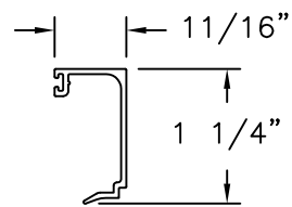
㉟ GLAZING BEAD 6063-T6 ALUMINUM 0.070" THICK
